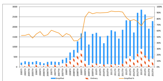
Graph III.7: Number of insolvency procedures by type
