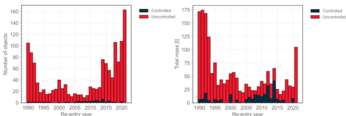
Figure 7: Amount of uncontrolled vs controlled de-orbiting
